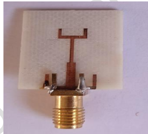
Figure 5: Fabricated Antenna – Bottom View
