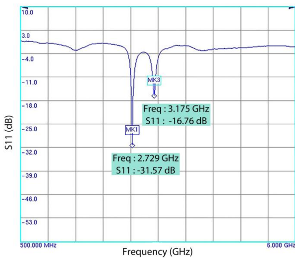
Figure 7: Return Loss for Diode – ON-OFF (10) state
