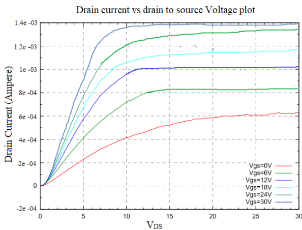
Figure 8: Drain current vs Drain to Source voltage plot
