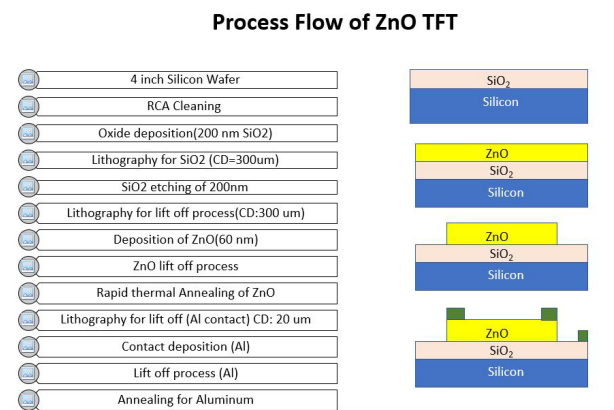
Figure 4: Complete process flow chart of ZnO TFT with tentative step-by-step design
