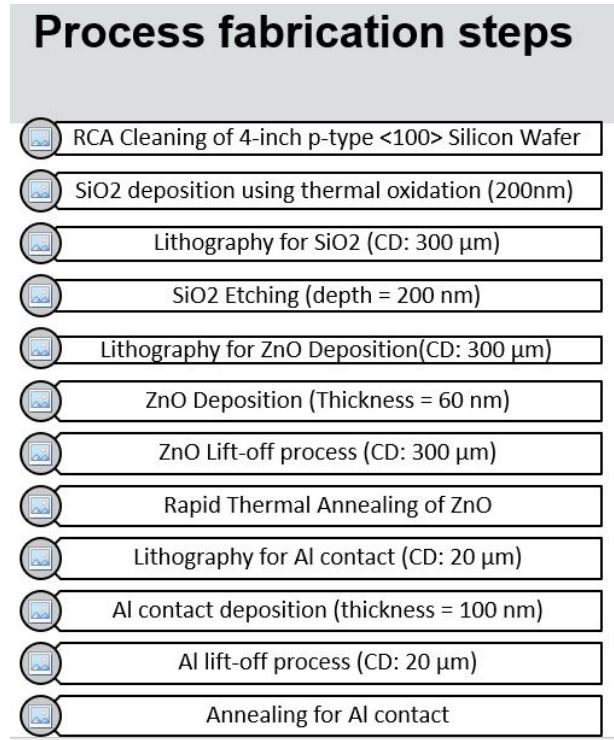
Figure 3: Process fabrication steps
