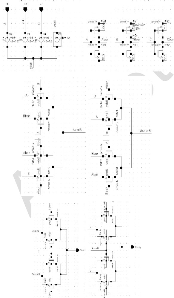
Figure 7: Proposed FA Cell 1 schematic design
