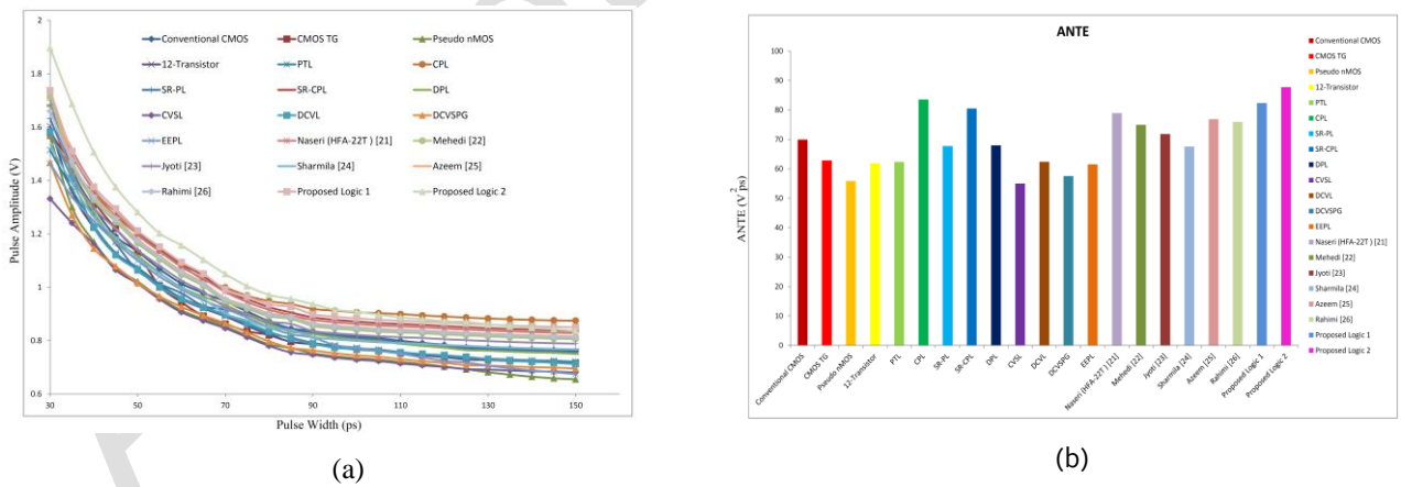
Figure 18: (a) NIC for various FA Cells (b) ANTE for various FA Cells
