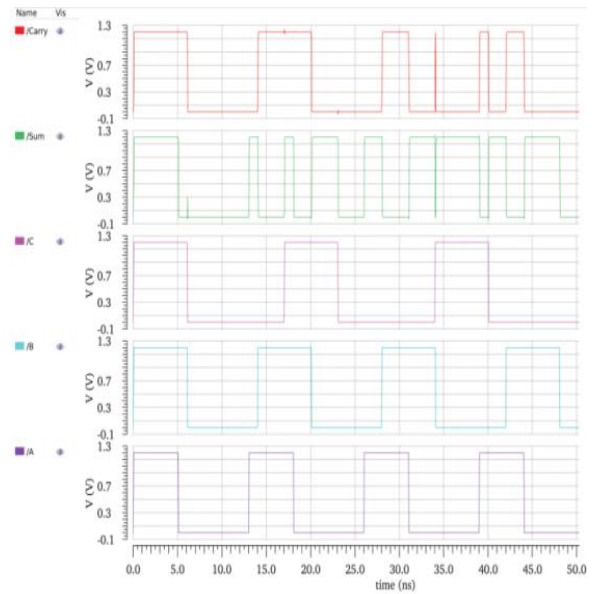
Figure 10: Proposed FA 2 Transient Analysis waveform
