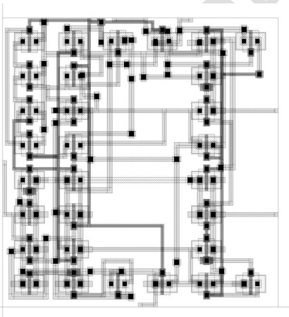
Figure 12: Proposed Full Adder 2 Layout
