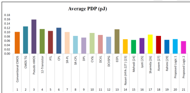
Figure 15: Average PDP Comparison of Various FA cells
