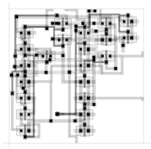
Figure 11: Proposed Full Adder 1 Layout
