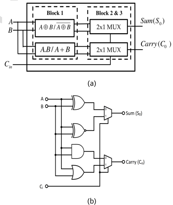
Figure 1 (a&b) : Full Adder Structure using Multiplexer based Alternative Logic
