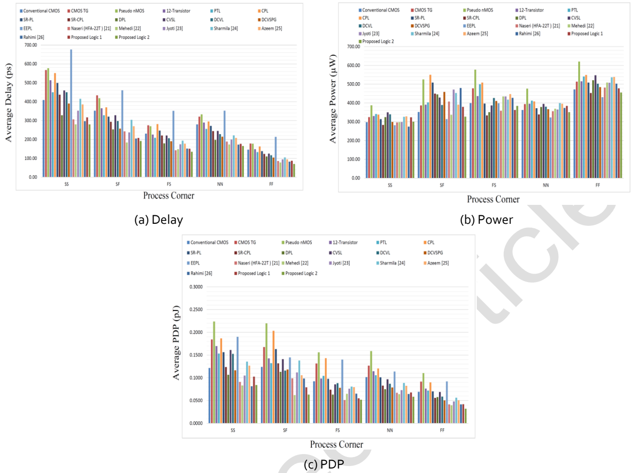
Figure 17: Various Process Corners vs Delay, Power and PDP
