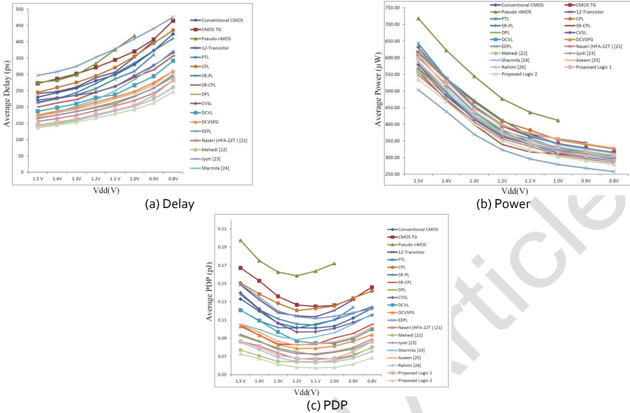
Figure 16: FA Cells simulation results for different V DD levels
