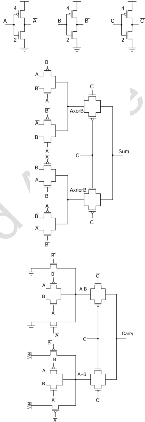
Figure 6: Proposed Hybrid Full Adder 2 based on alternative logic using DPL
