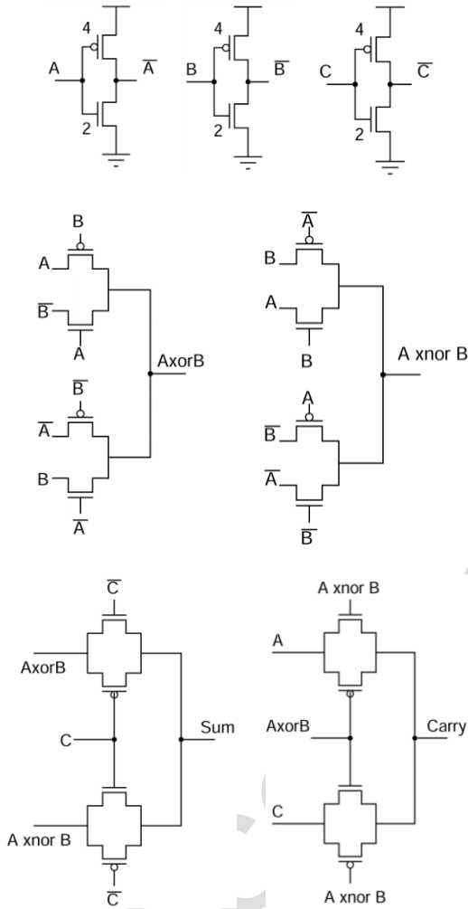
Figure 5: Proposed alternative logic based Full Adder 1 using DPL
