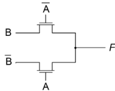
Figure 2: EX-OR Logic Gate implementation using PTL
