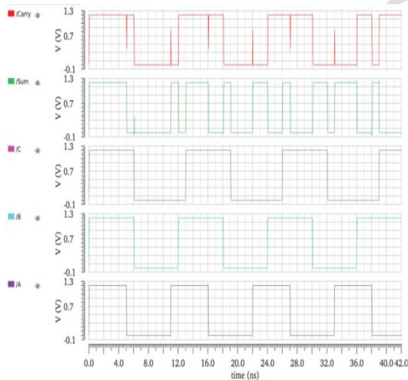
Figure 9: Proposed FA 1 Transient Analysis waveform
