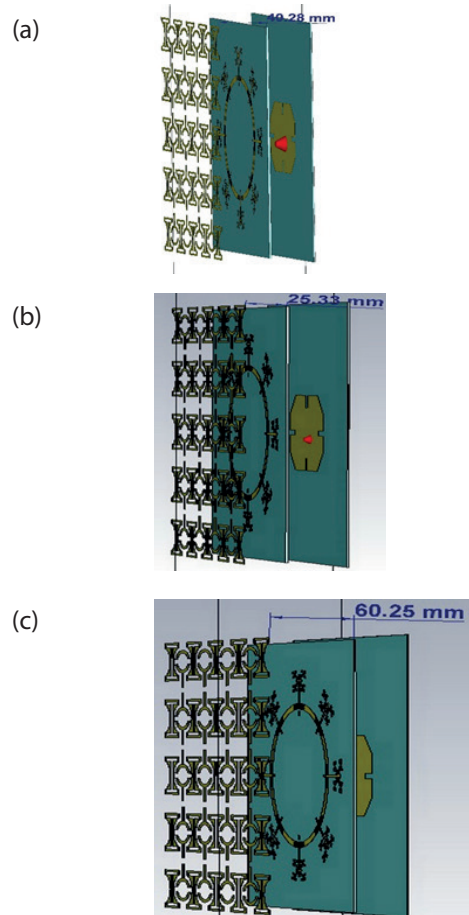
Figure 7: Distances of the MTS structure a) case 1 b) case 2 c) case 3
