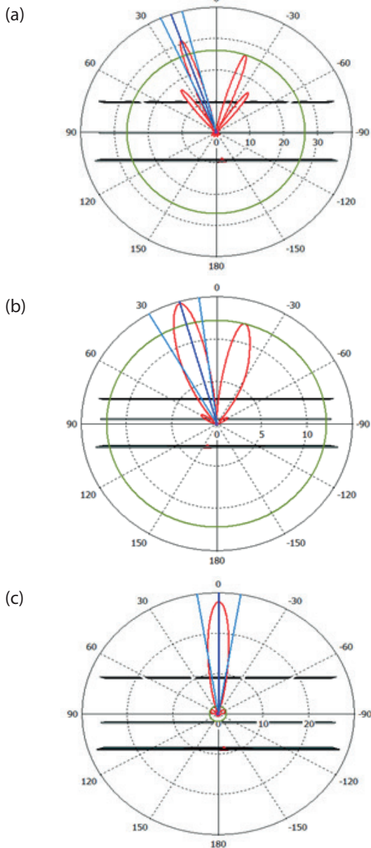
Figure 9: The radiation pattern of antenna at a) 4.4 GHz b) 3.1GHz c) 3.3 GHz
