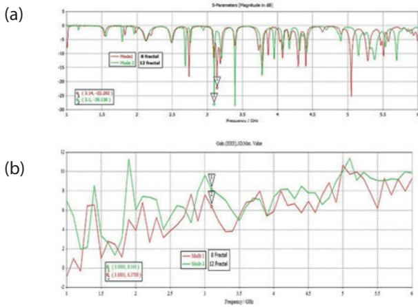
Figure 6: The CRLH structure (second layer) a) reflection coefficient results in b) gain result.
