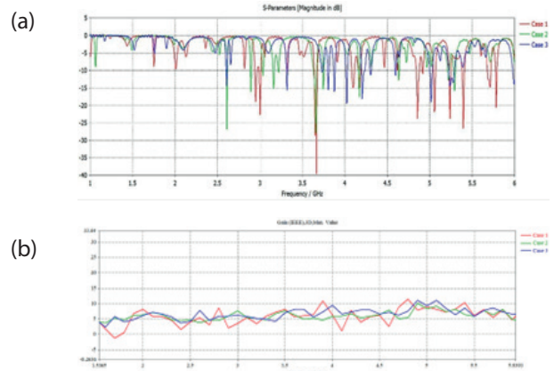
Figure 4: The parametric study of patch antenna (First Layer) a) reflection coefficient of antenna b) the gain of patch antenna.
