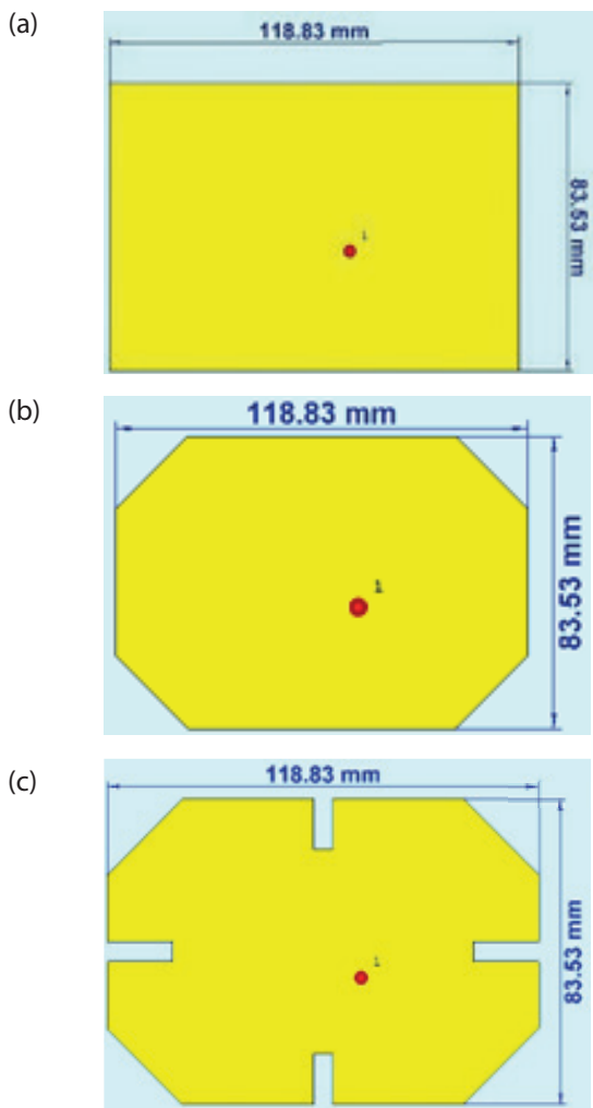
Figure 3: The modeling of patch antenna a) the rectangle patch b) the cutting edge of rectangle c) the antenna proposal.
