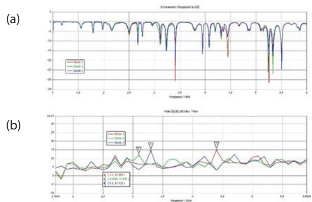
Figure 8: The result of MTS a) the Reflection coefficient of antenna b) the gain
