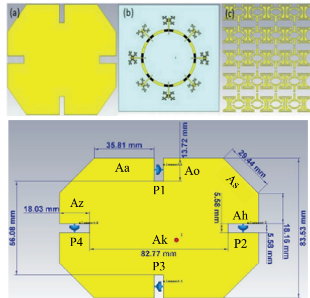
Figure 2: The proposed antenna structure with geometrical details.
