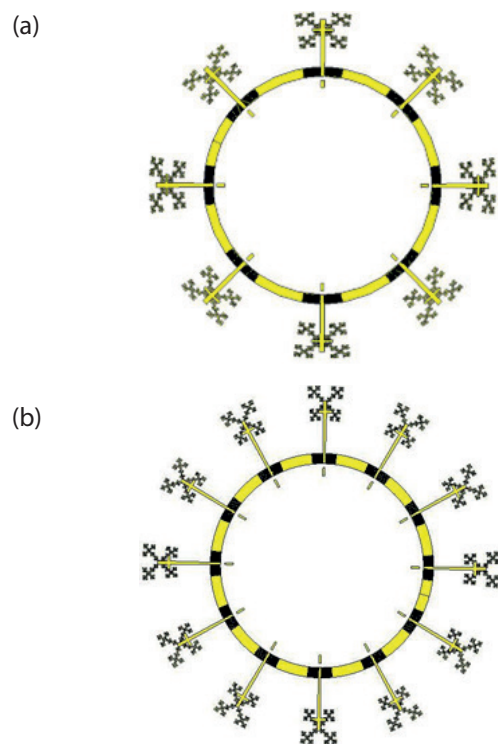
Figure 5: The CRLH structure (second layer) a) the 8 Fractal b) 12 Fractal.
